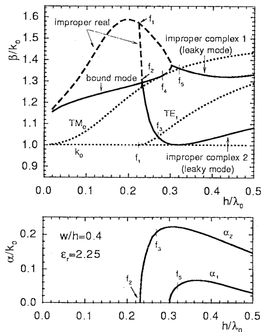
Fig. 2 The normalized phase and leakage constants for the slotline with w/h=0.4 and \epsilon_r=2.25 as a function of normalized frequency ( h/\lambda_0 ).
